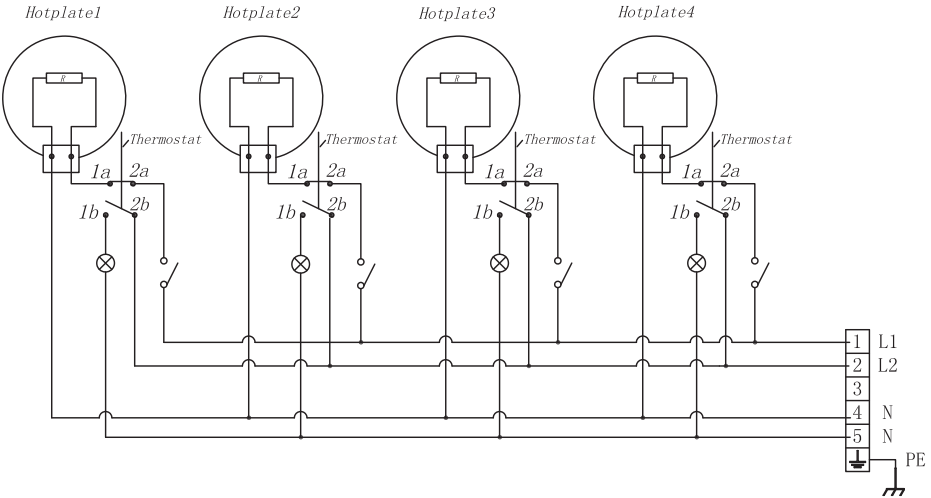
The wiring diagram
