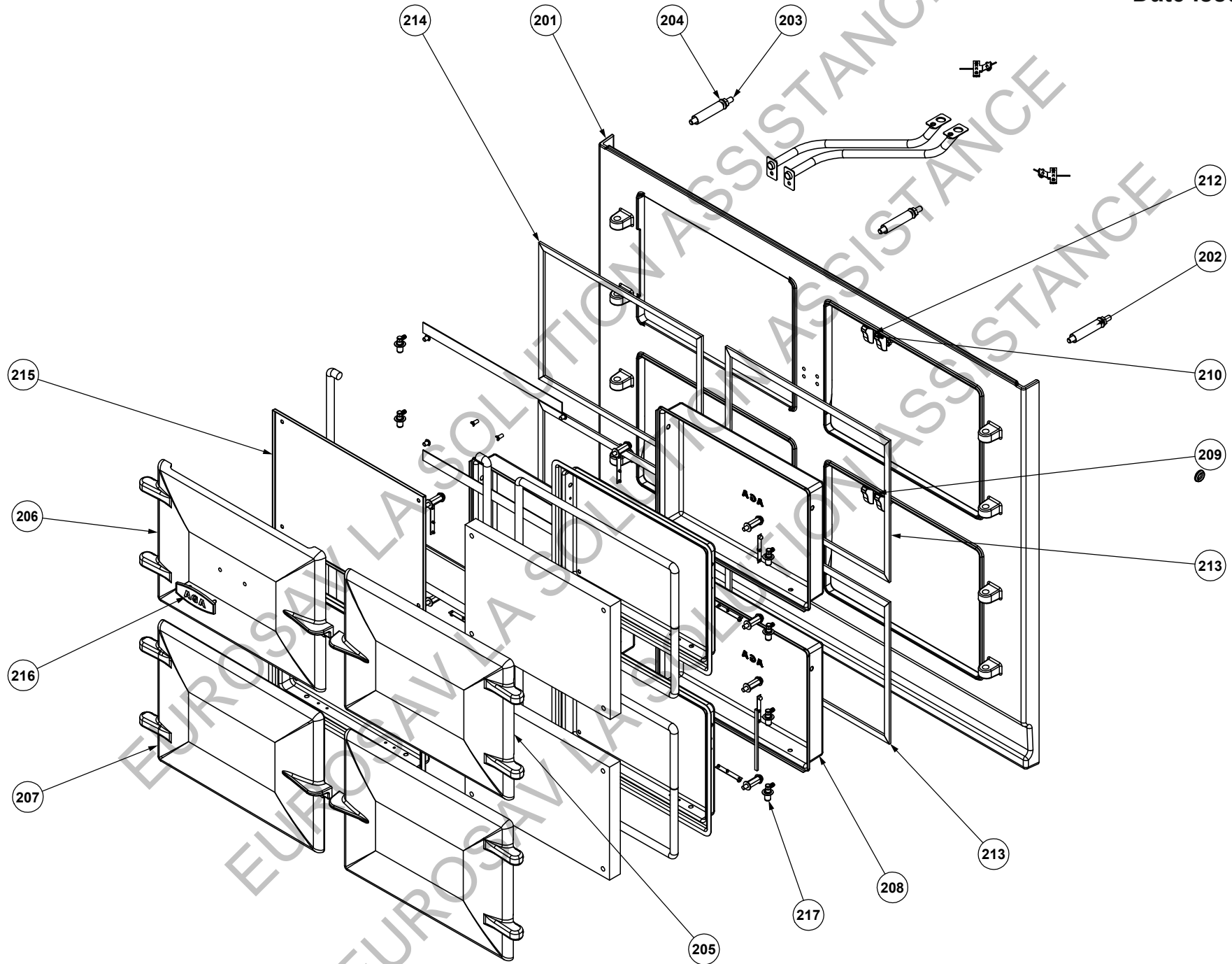
AE1M281224 eR7 FRONT PLATE ASSEMBLY
