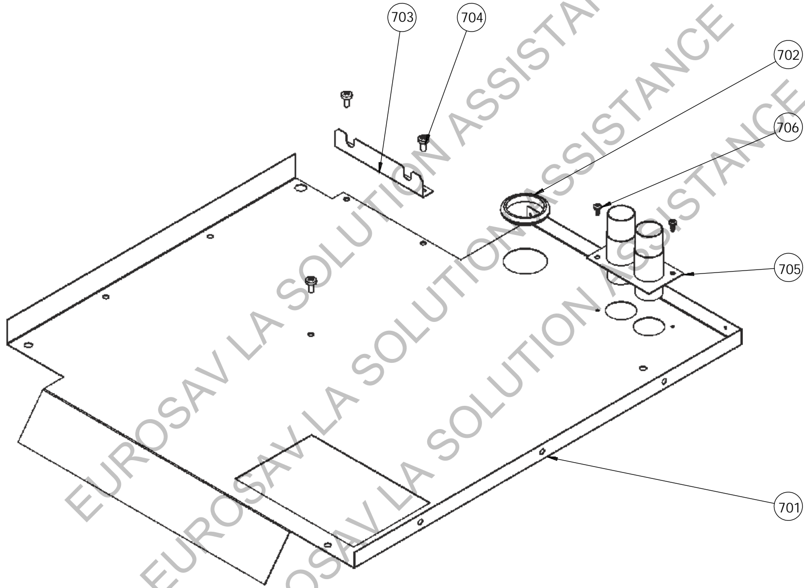
eR3 90 DIVIDER PLATE ASSEMBLY
