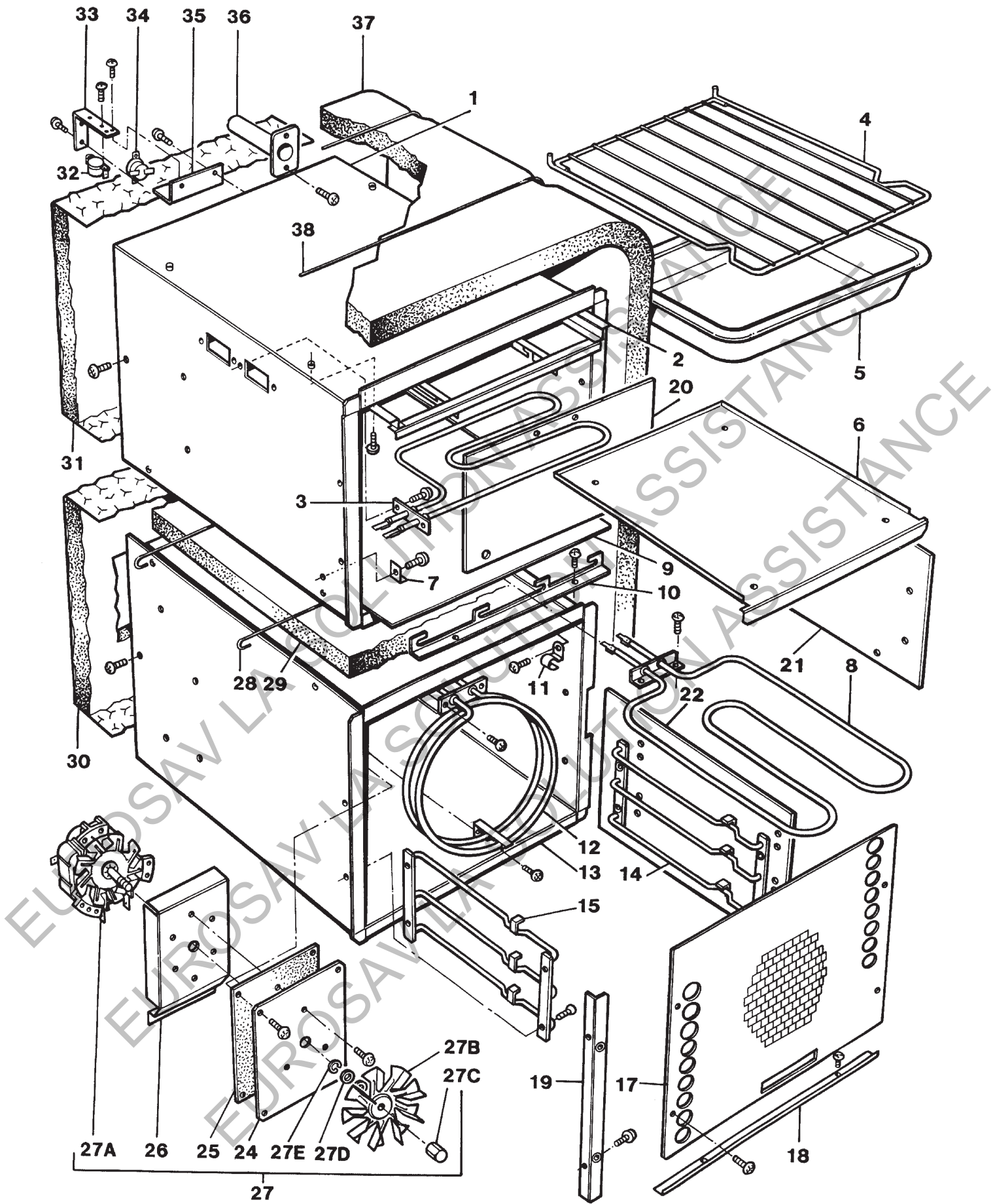
AGA ELECTRIC MODULE TOP & BOTTOM OVEN ASSEMBLIES
