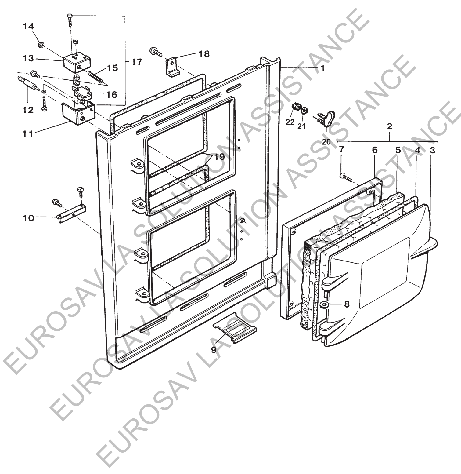
AGA ELECTRIC MODULE FRONT PLATE & DOOR ASSEMBLY
