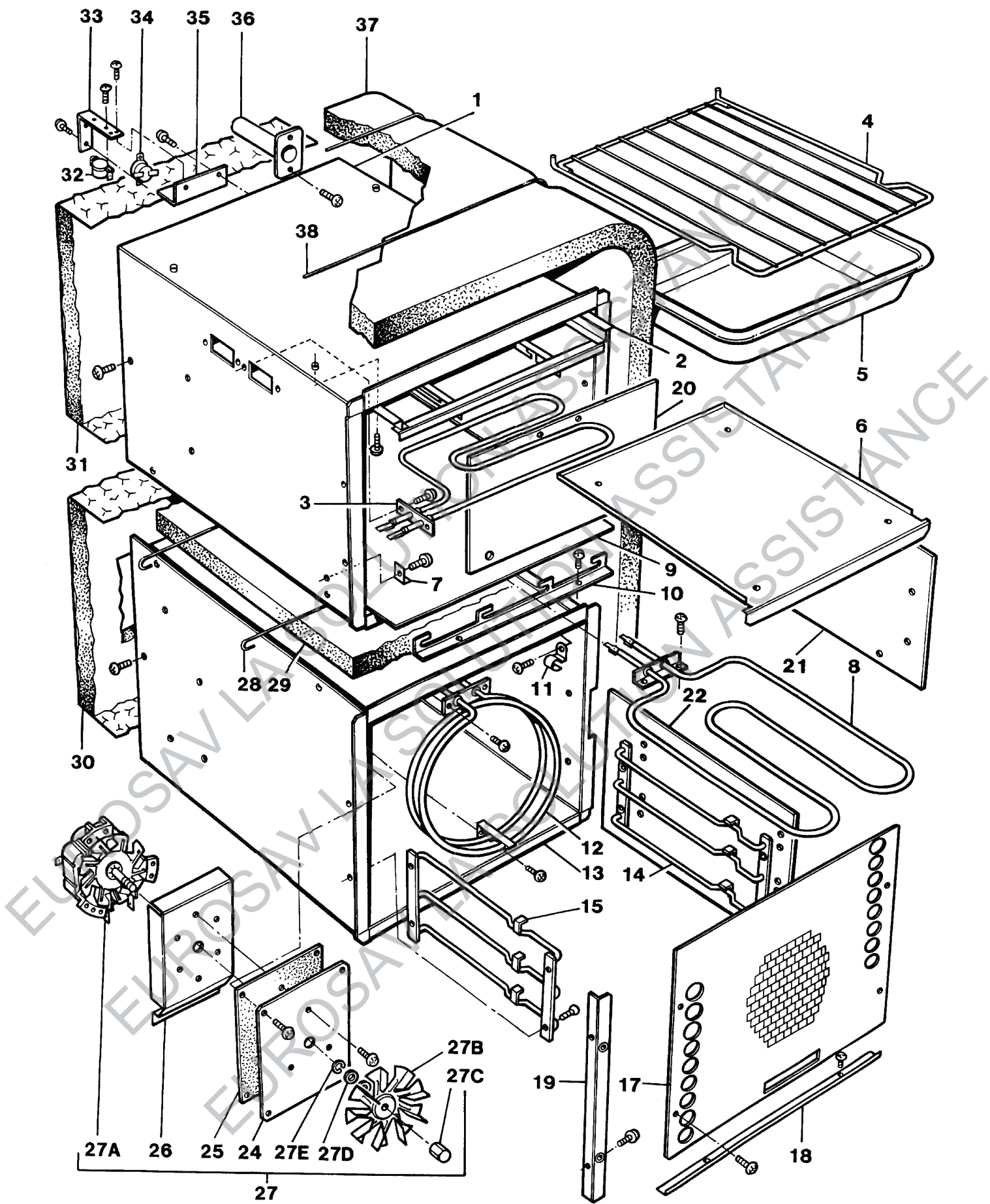
AGA ELECTRIC COMPANION TOP & BOTTOM OVEN ASSEMBLIES
