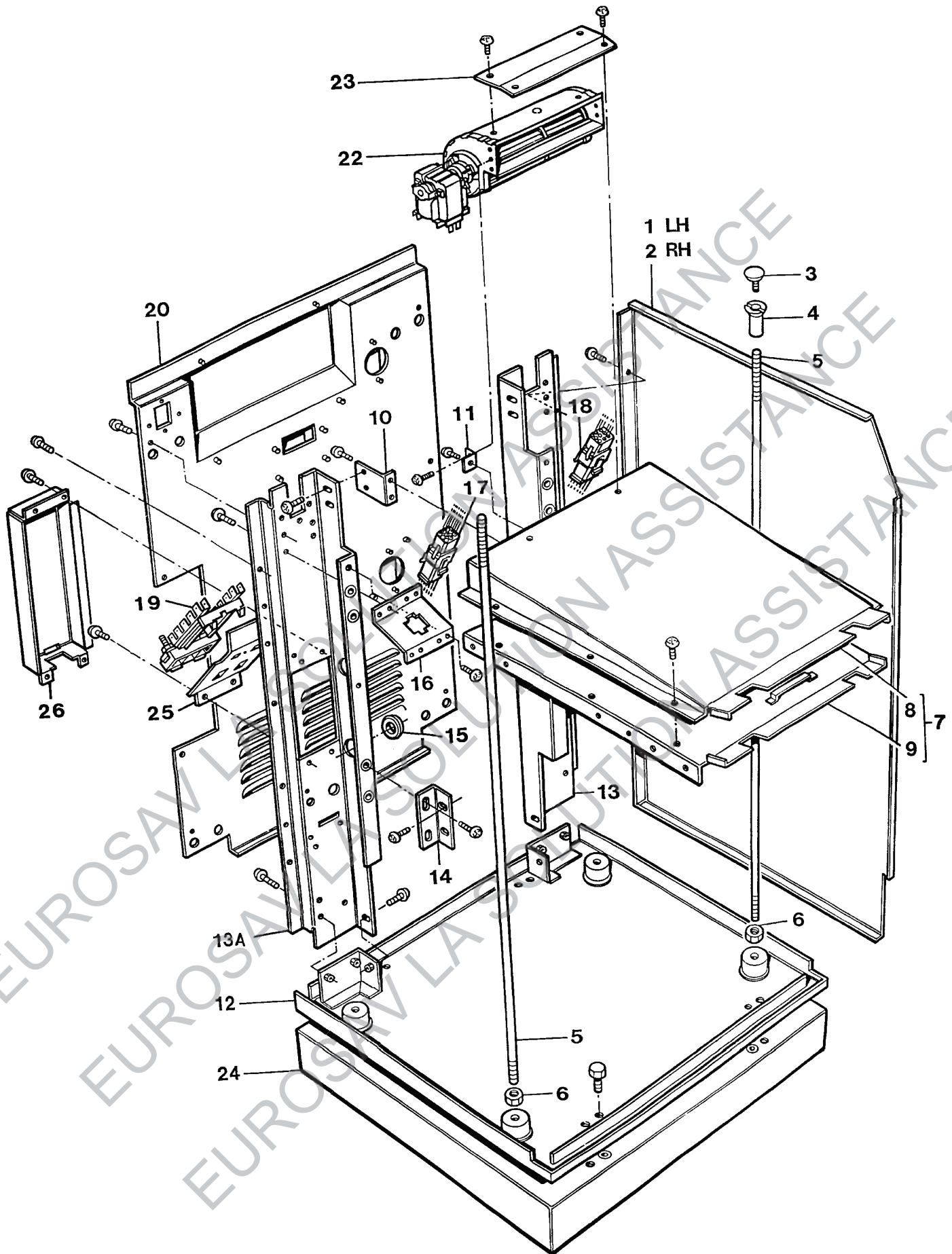
AGA ELECTRIC COMPANION (UP TO M01-086) BASE, BACK PLATE & COOLING DUCT ASSEMBLY
