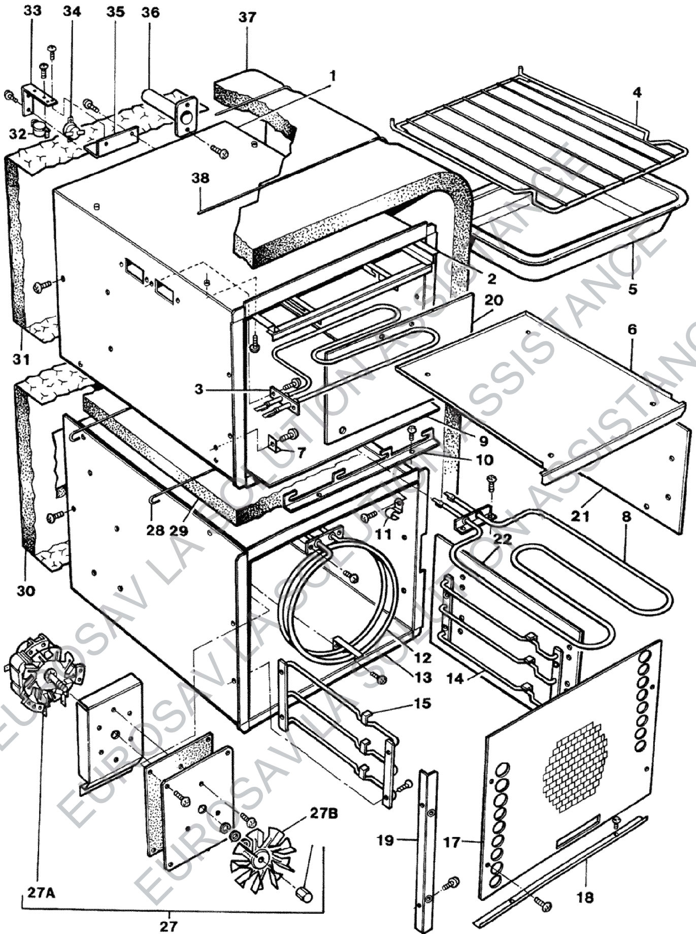
TOP & BOTTOM OVEN ASSEMBLIES AGA GAS COMPANION - FFD
