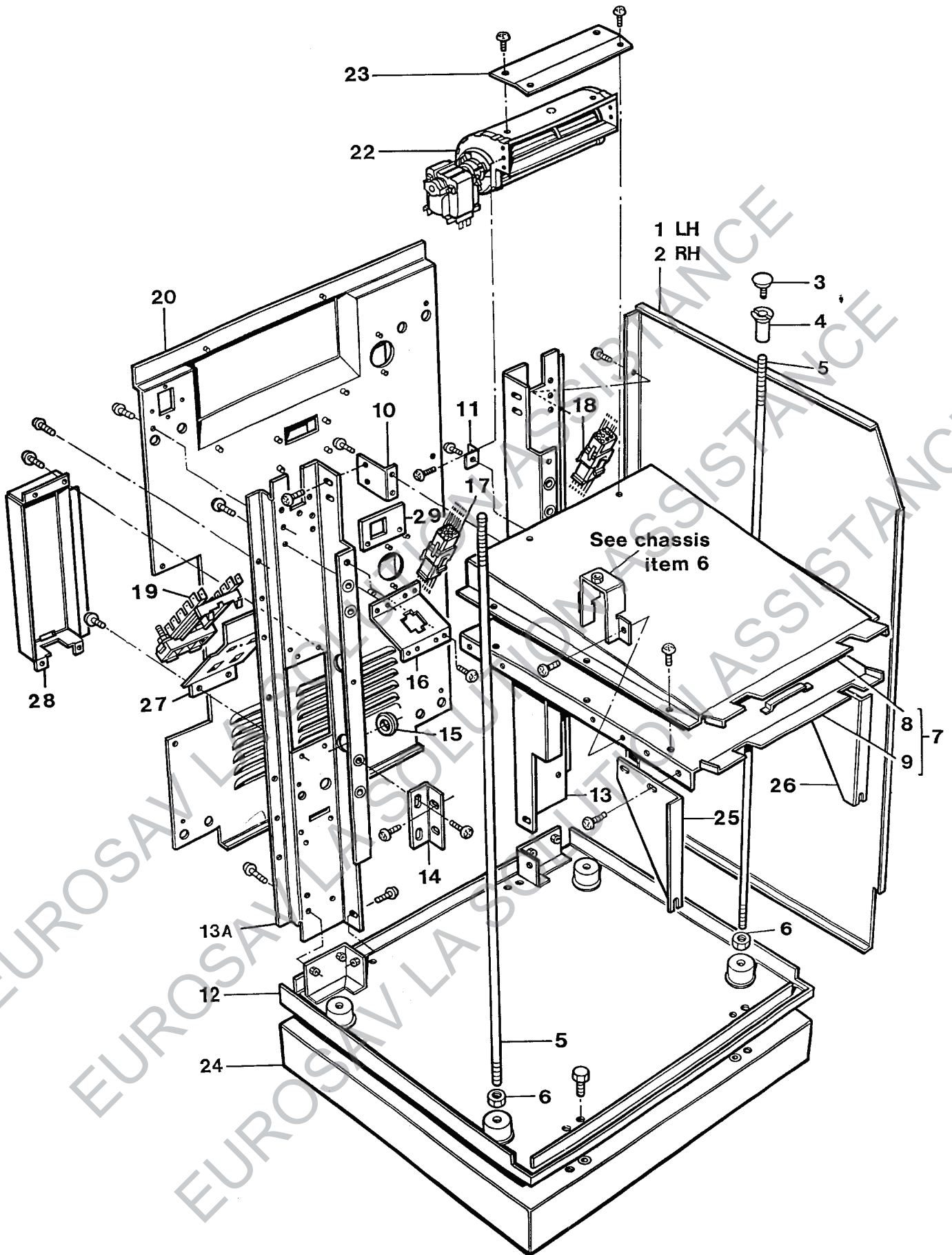
BASE, BACK PLATE & COOLING DUCT ASSEMBLY AGA GAS COMPANION - FFD (UP TO M01-086)
