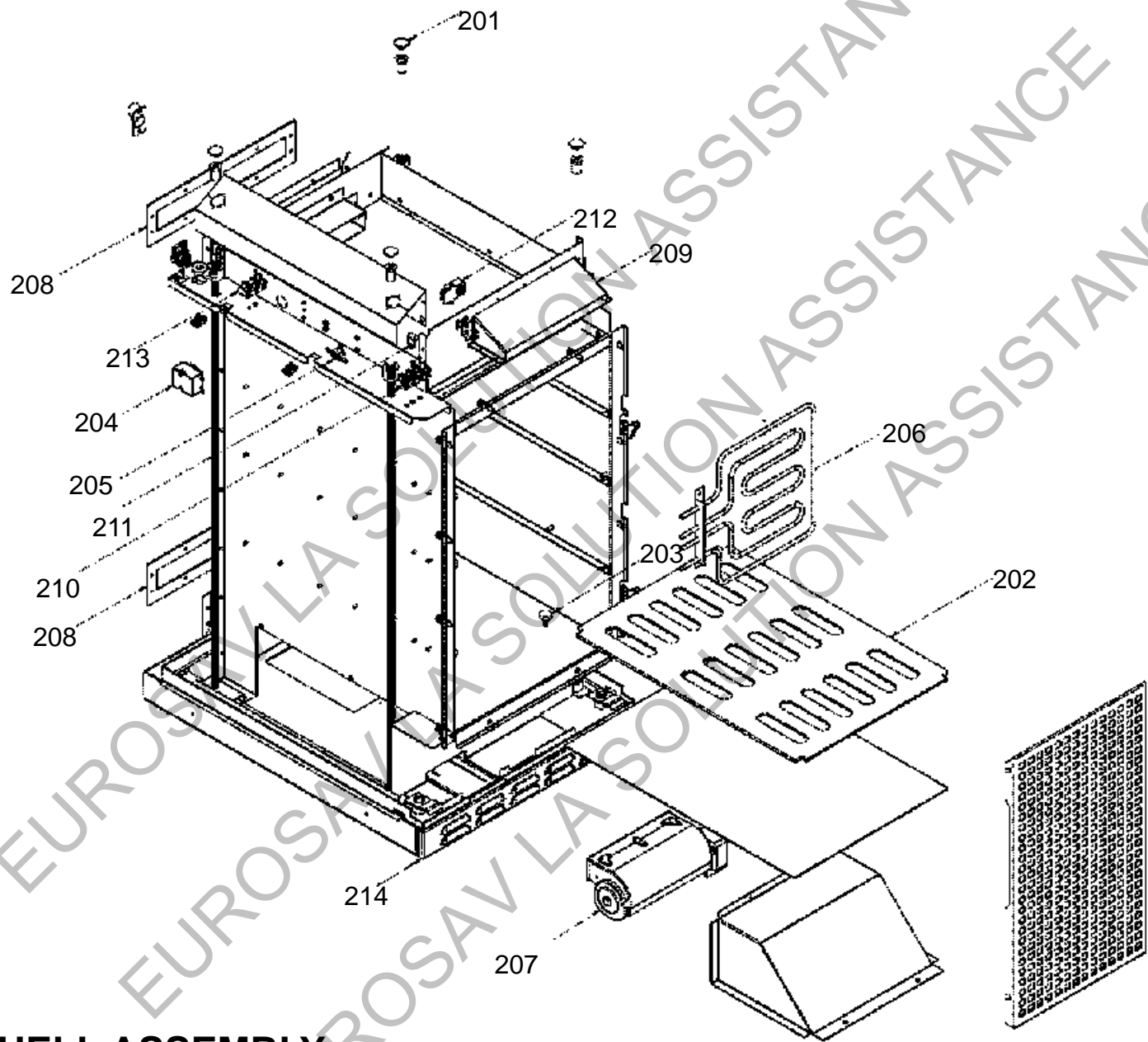
INNER SHELL ASSEMBLY
