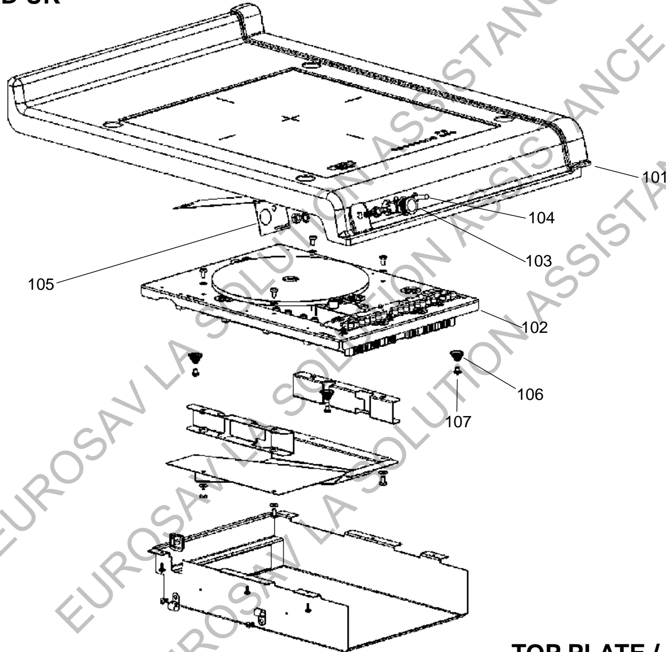
TOP PLATE / HOB ASSEMBLY
