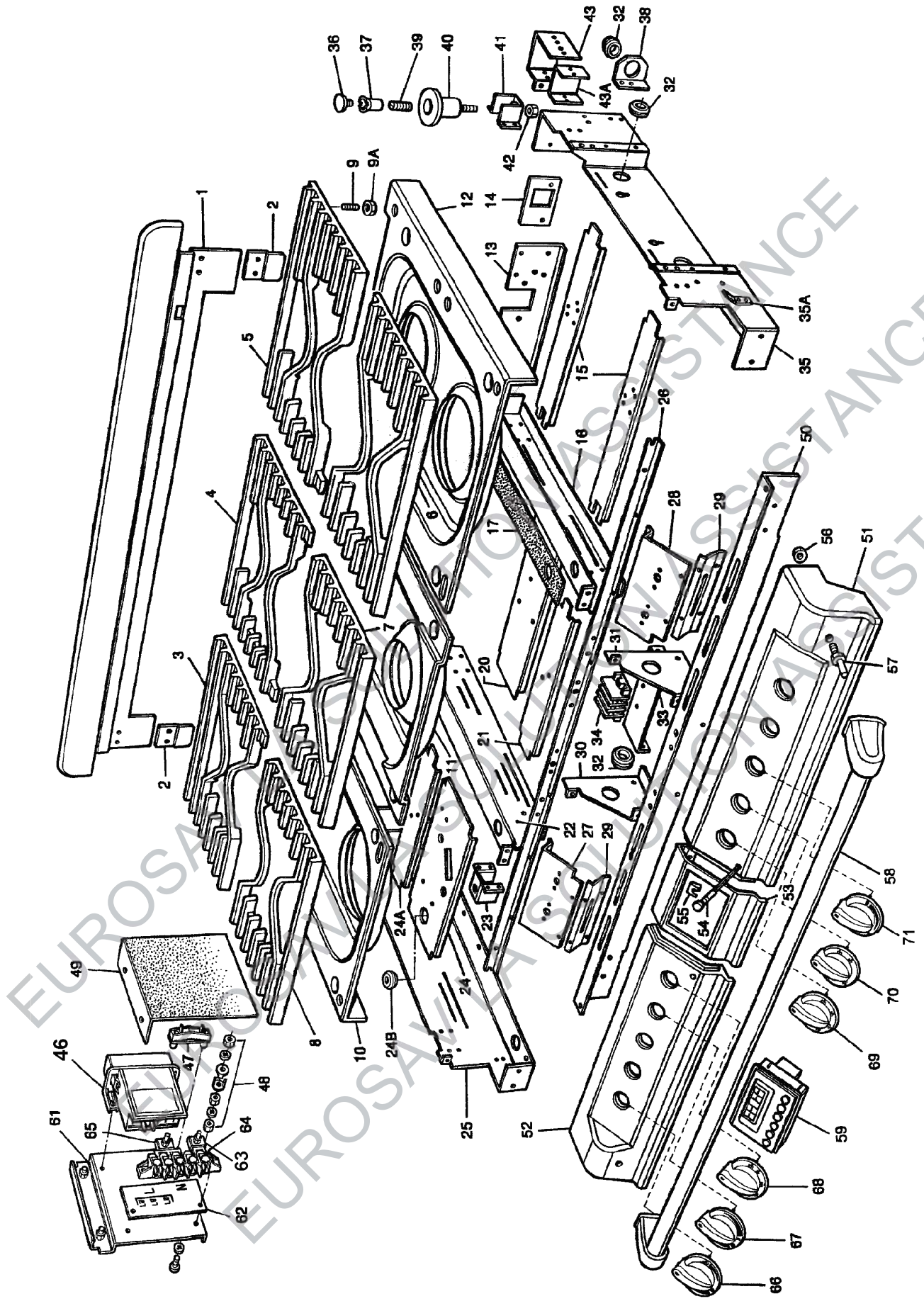
AGA SIX-FOUR SERIES - DC6 (WITH FFD'S) (FROM NP04-019) TOP PLATE AND HOTPLATE FRAME
