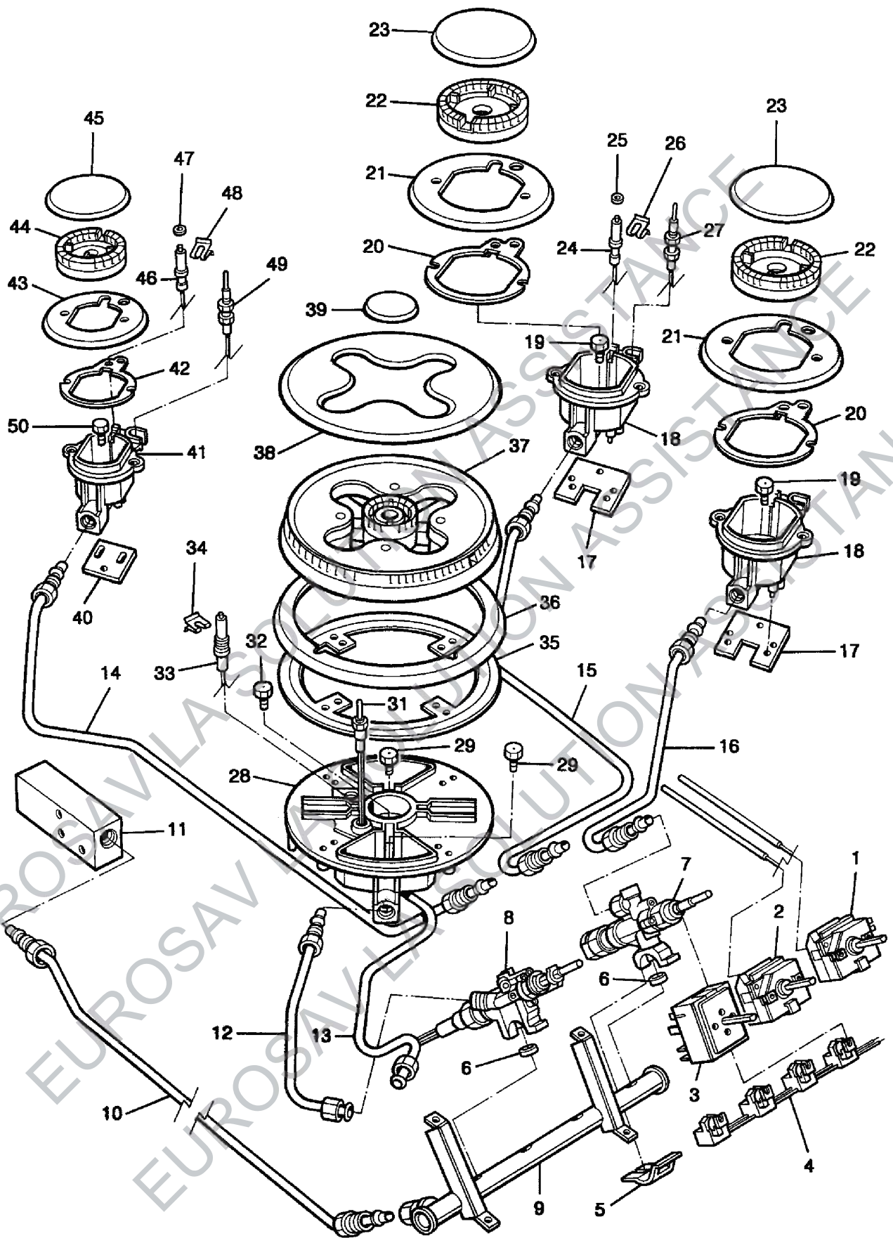
AGA 4-2 (WITH FFD'S) HOTPLATE BURNER PARTS
