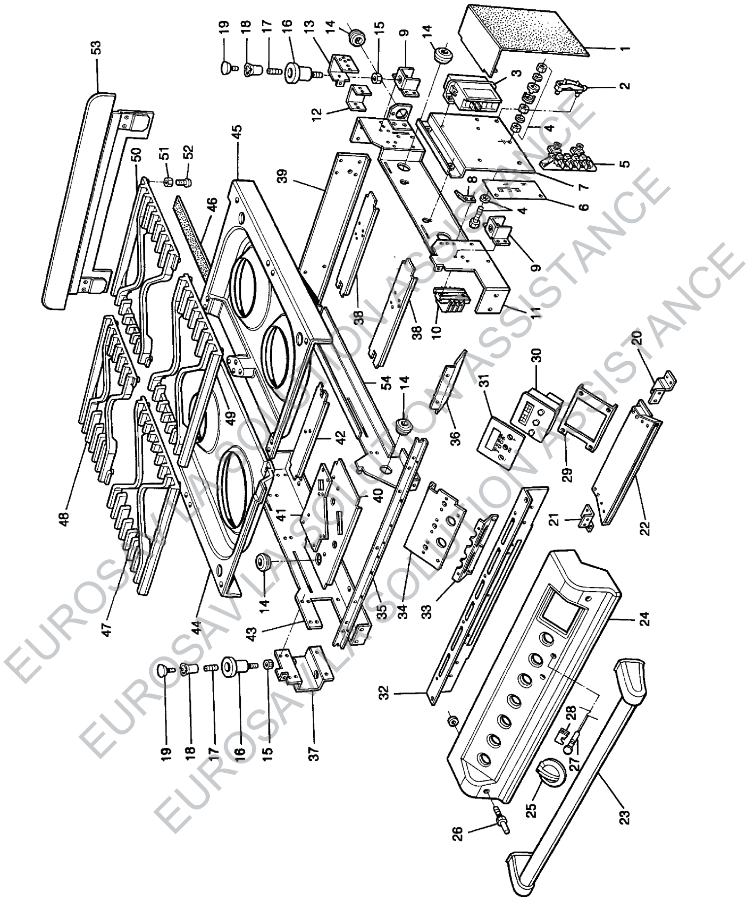
AGA 4-2 (WITH FFD'S) TOP PLATE AND HOTPLATE FRAME
