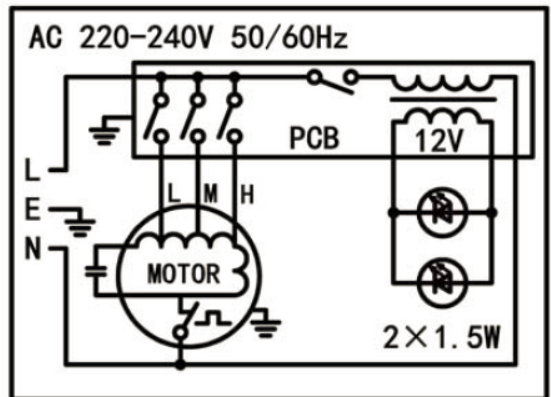
ELECTRICAL CONNECTION DIAGRAM
