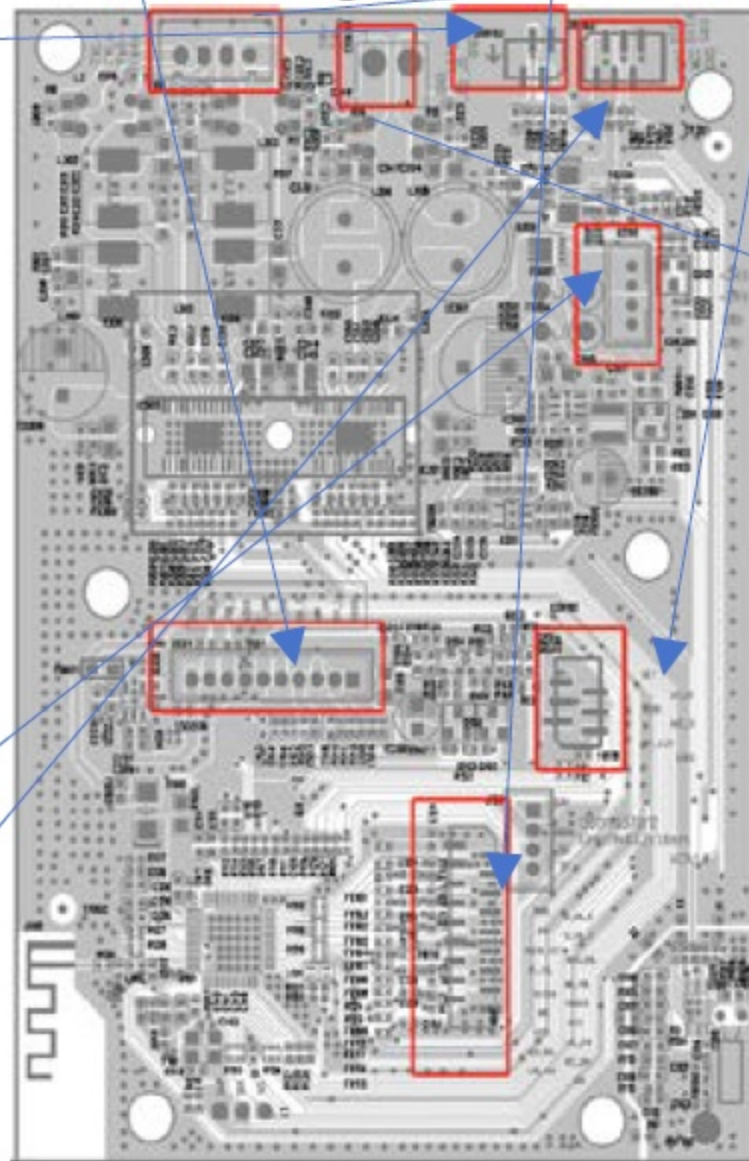
Decoding board PCBA
