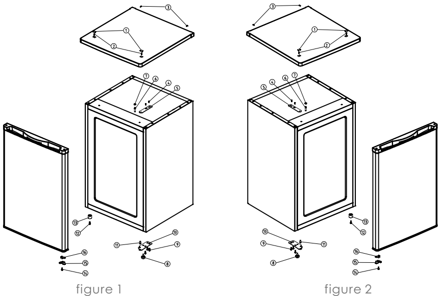
Figure 1: Represents position of components prior to door reversal
