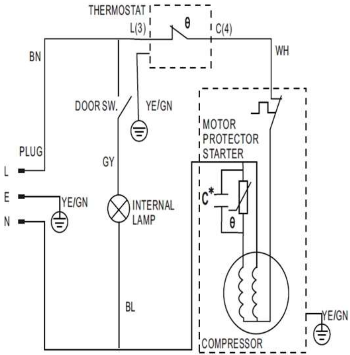
C* : The capacitor is optional according to different compressor model
