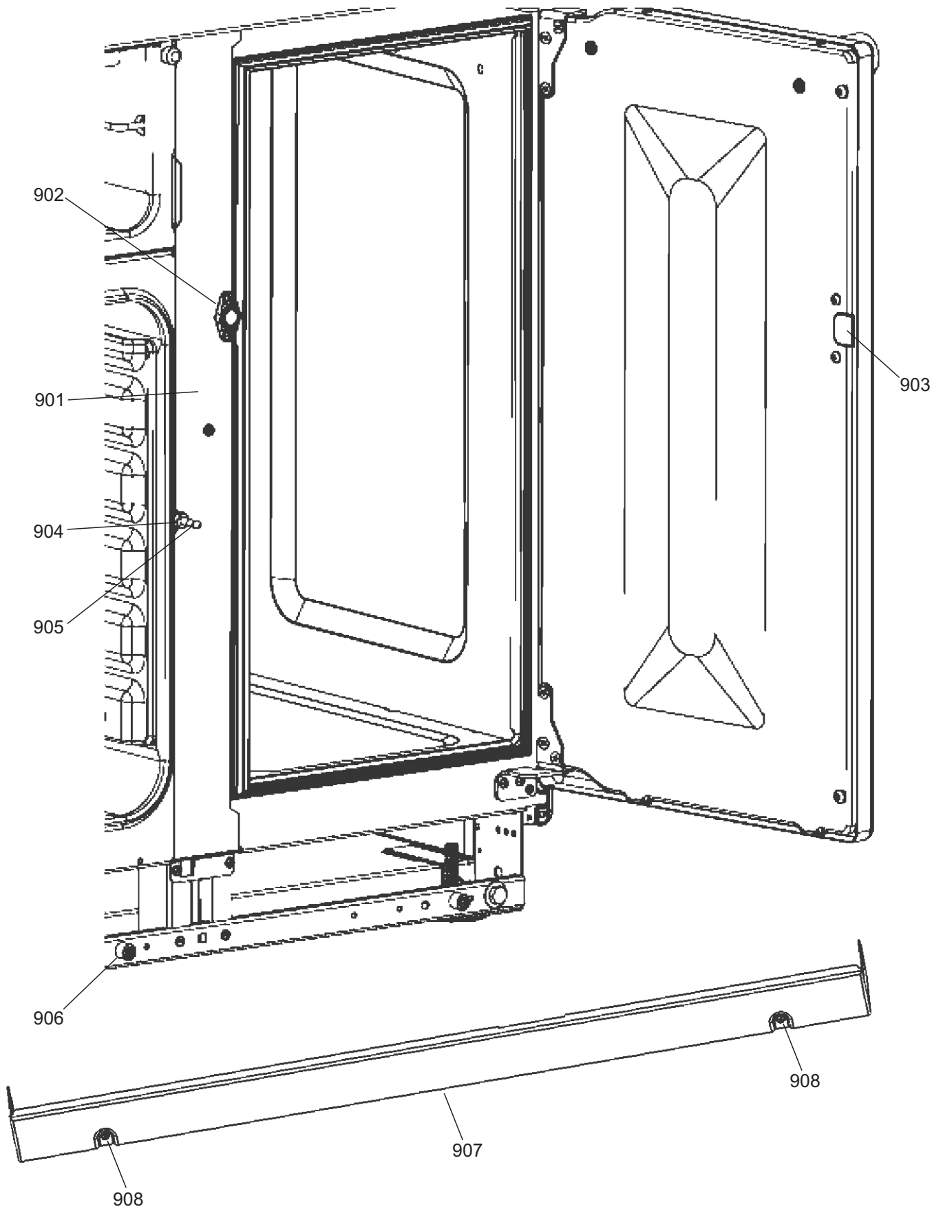
CHASSIS ASSEMBLY
