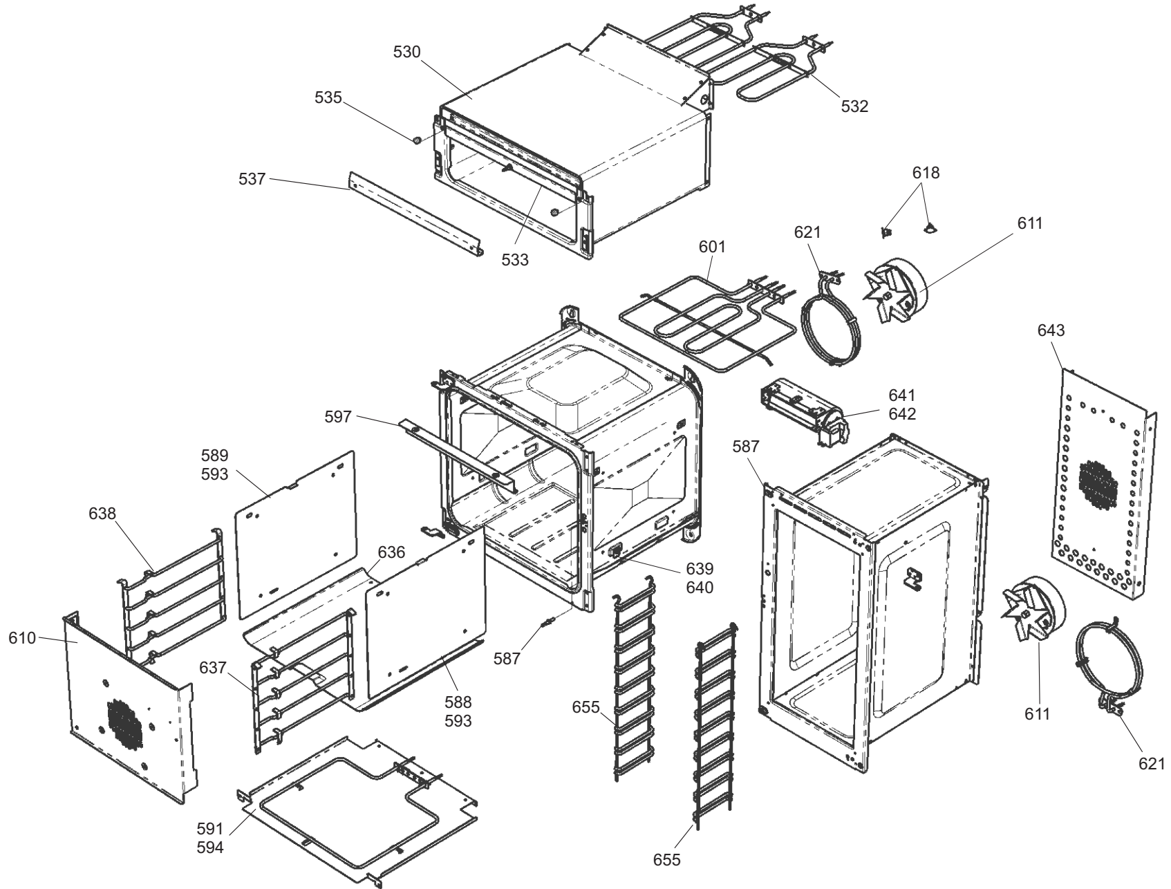
LH OVEN - RH OVEN AND GRILL CHAMBER
