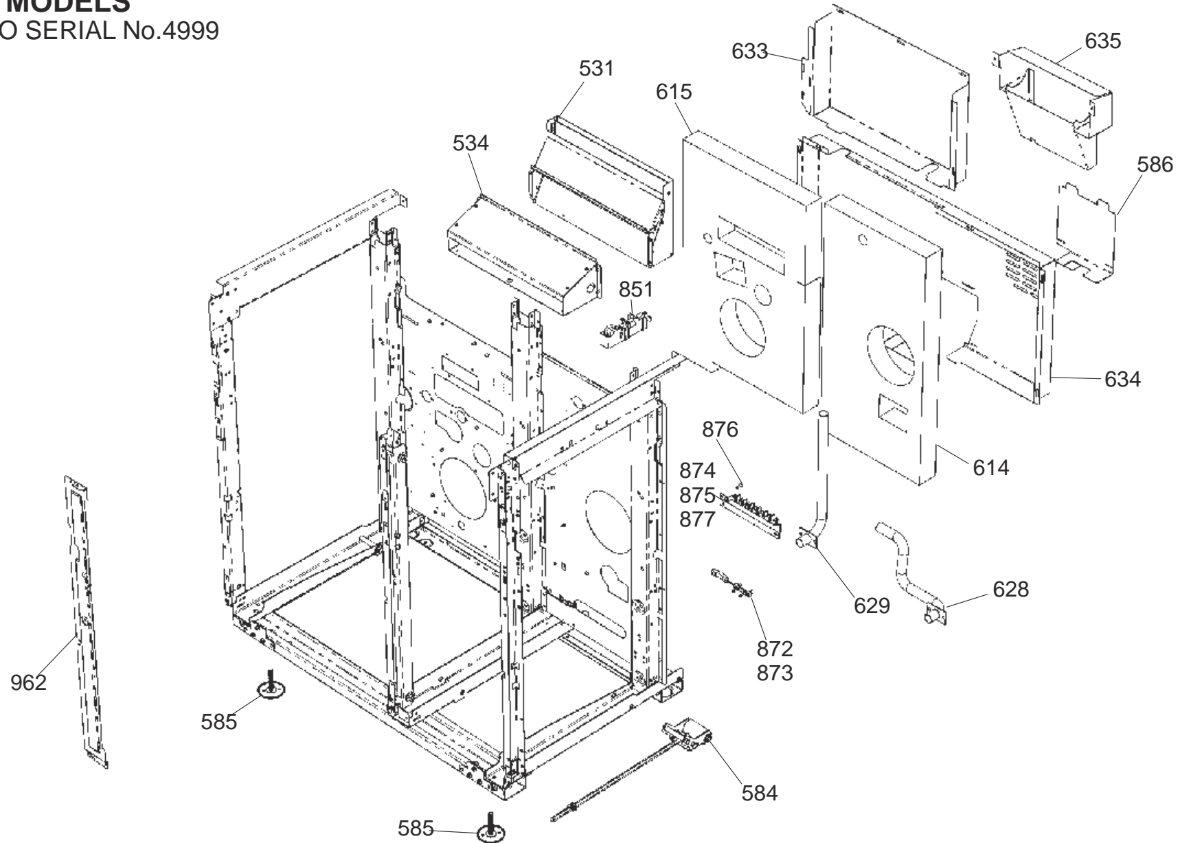
CHASSIS AND FRAME ASSEMBLY
