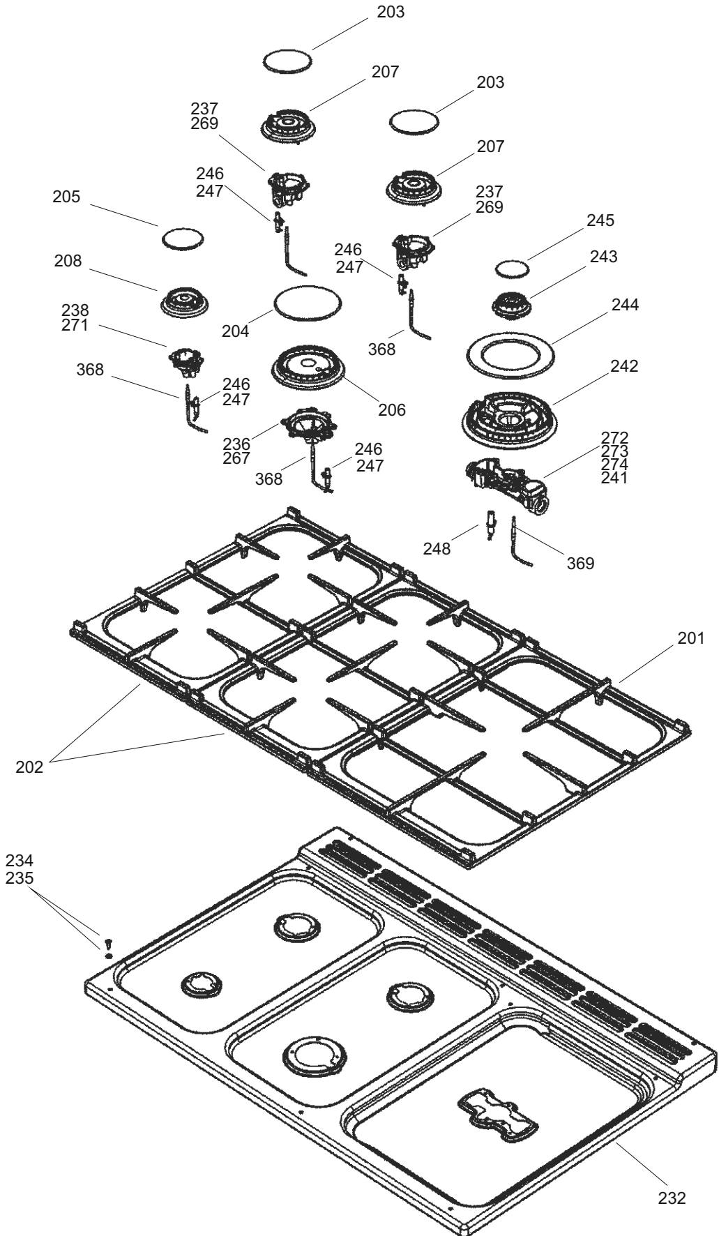
PAN SUPPORTS BURNERS & HOTPLATE ASSEMBLY
