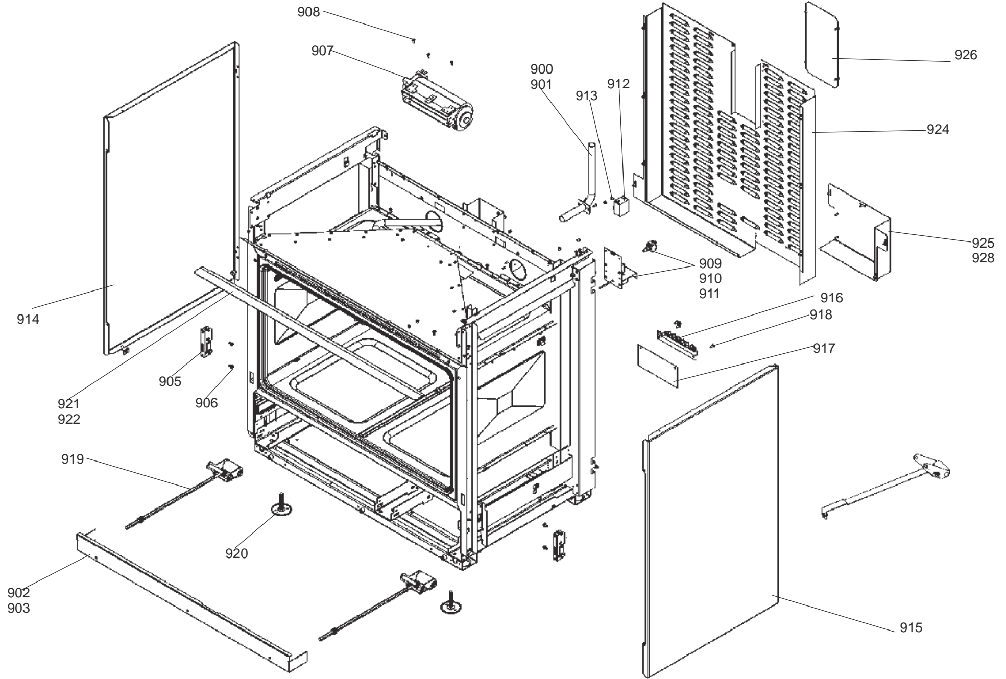
CHASSIS AND FRAME ASSEMBLY
