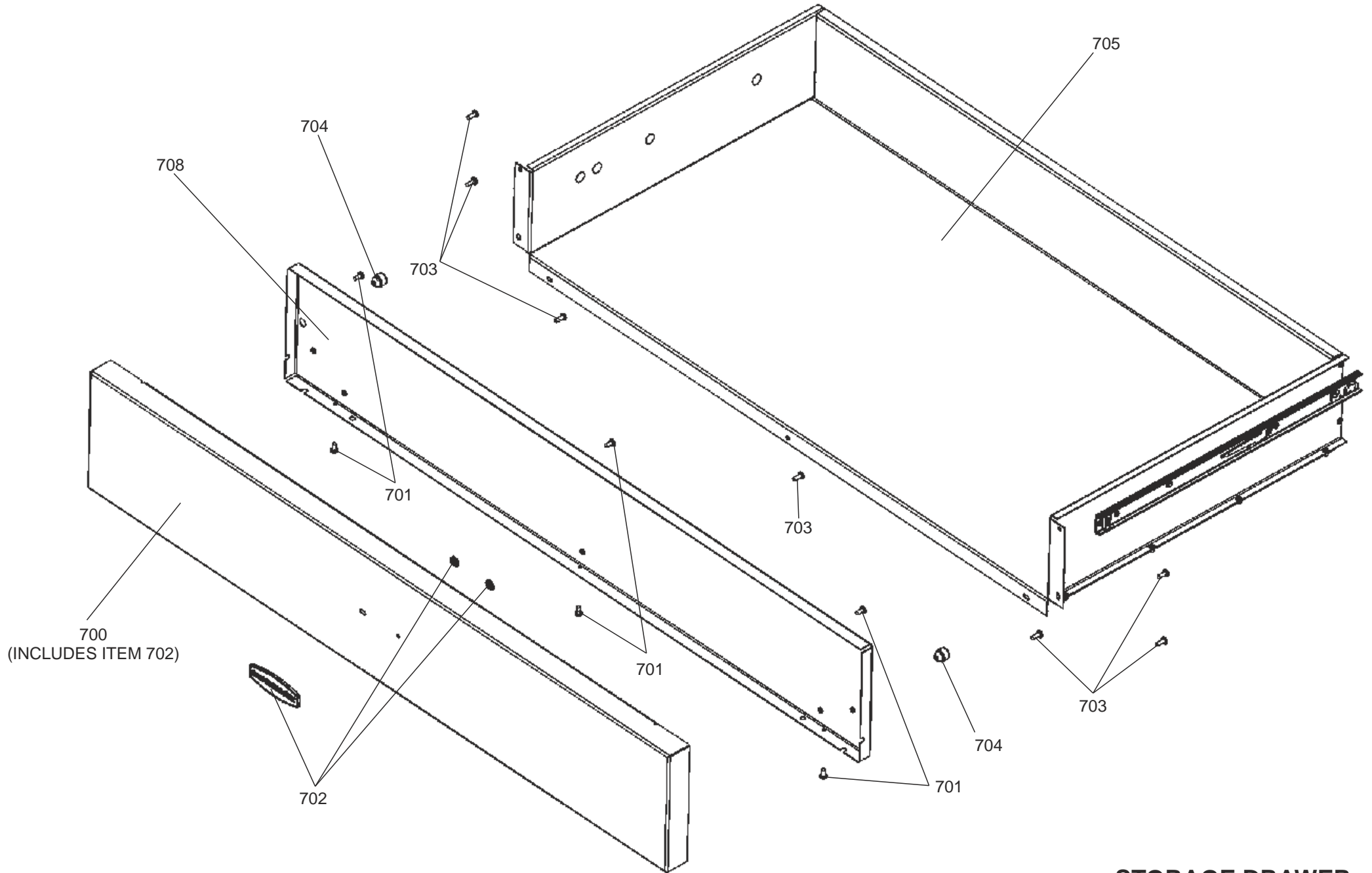
STORAGE DRAWER
